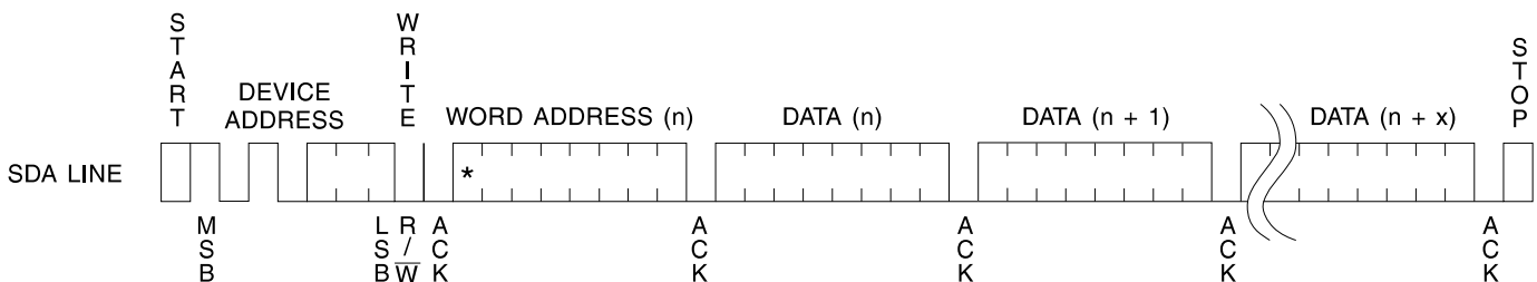
Figure 3. Page Write
